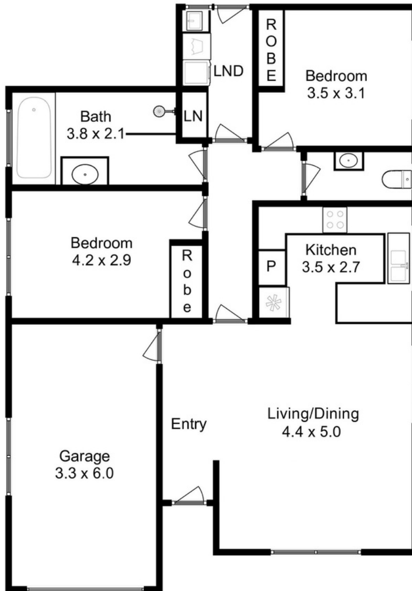
FLOOR PLAN
