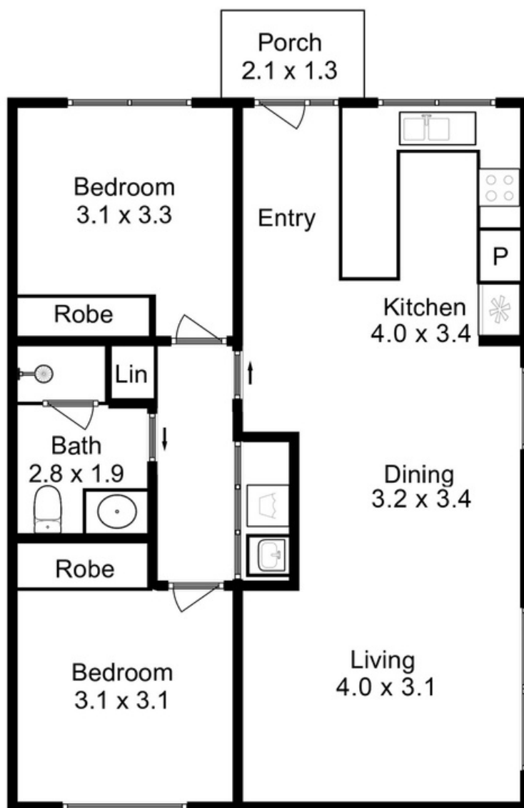
FLOOR PLAN
