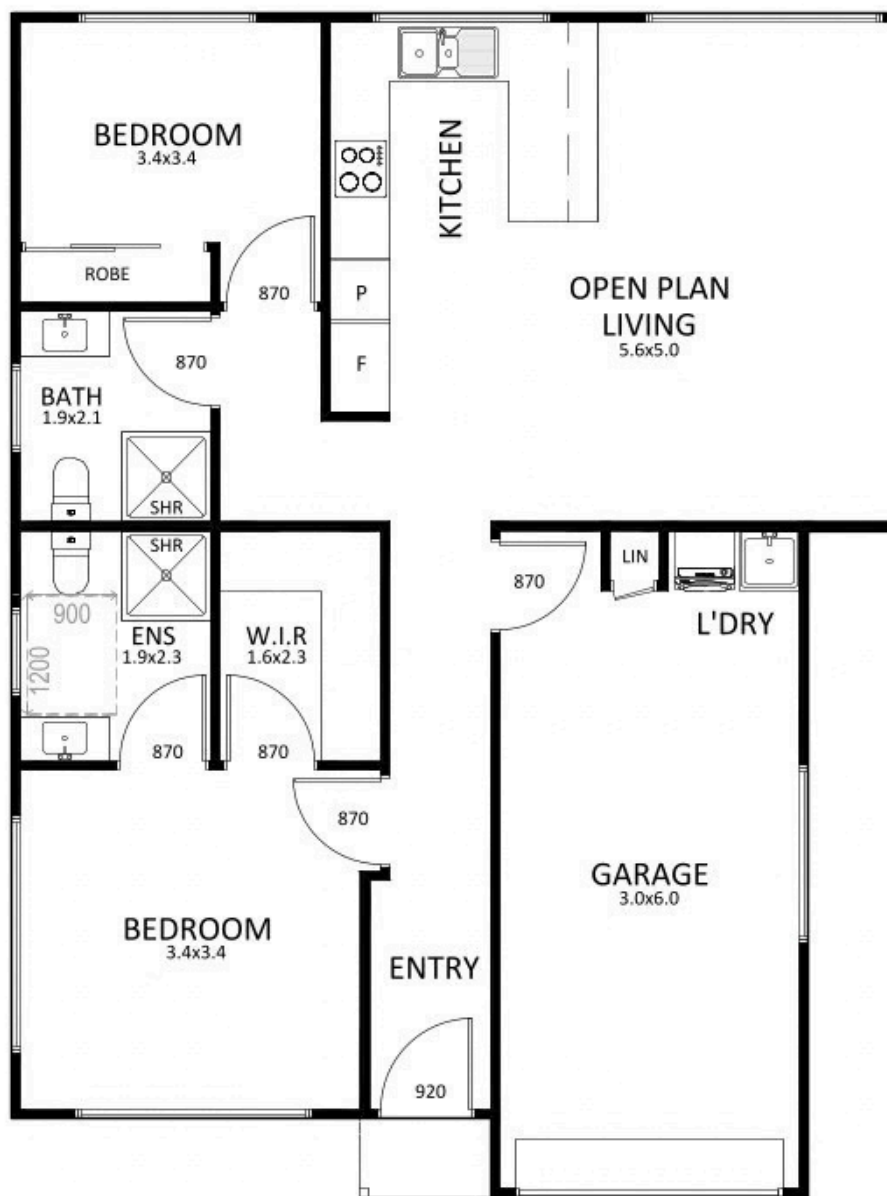
FLOOR PLAN
