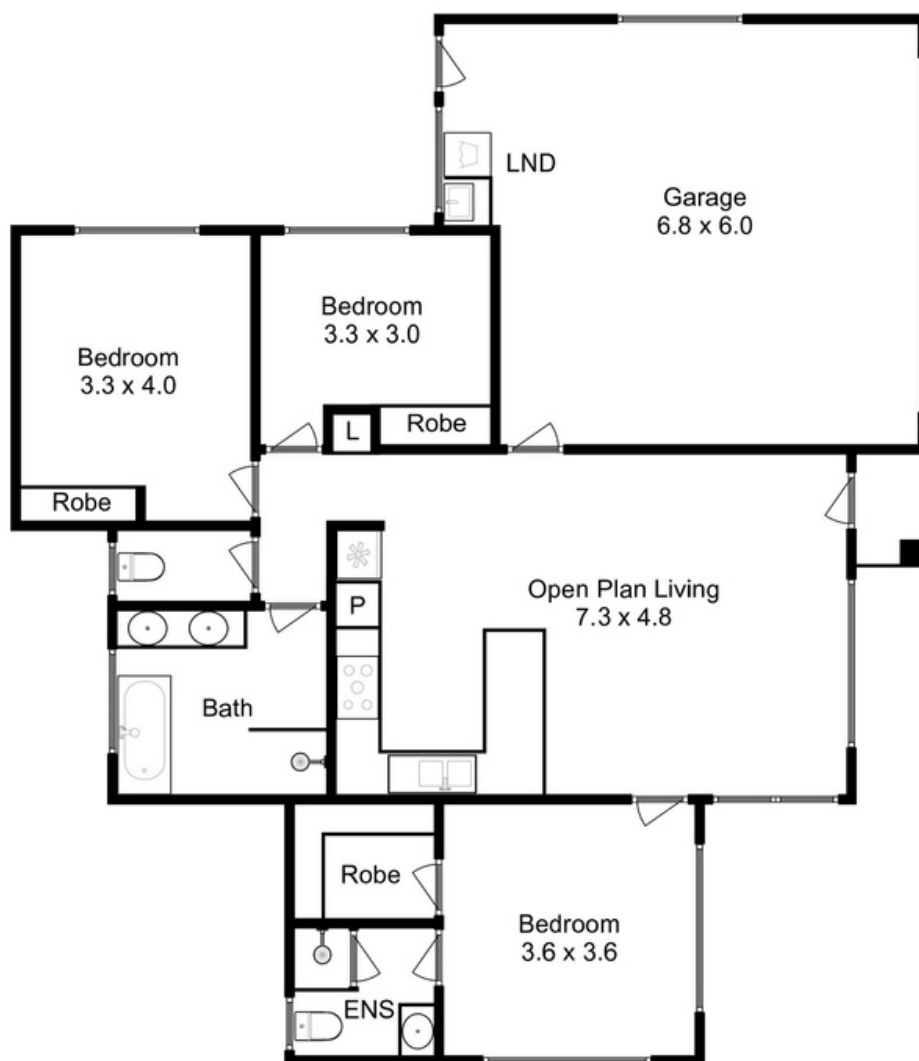
FLOOR PLAN
