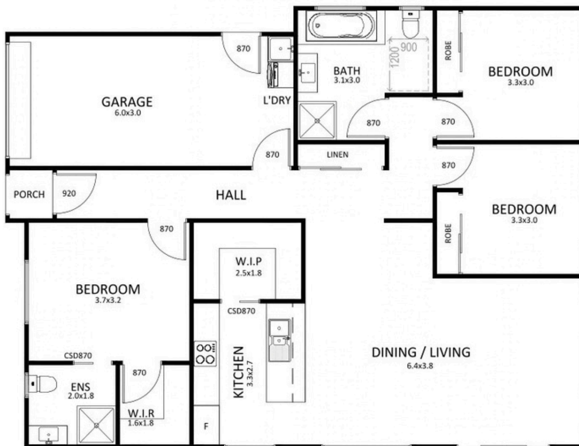
FLOOR PLAN
