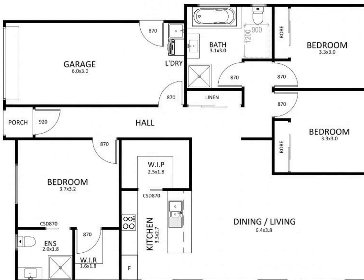
FLOOR PLAN
